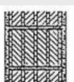
Figure 9: Common building construction types in old buildings (Manual for Energy Advisors)
